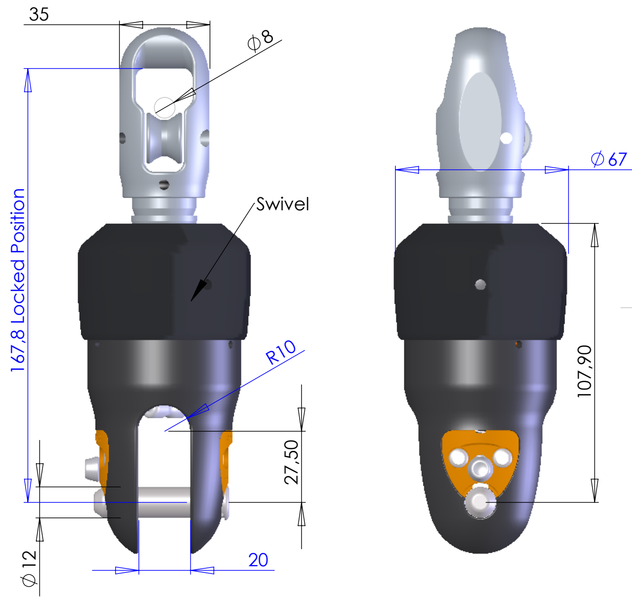
PF320600 + PF410953 Lashing 0° from halyard
