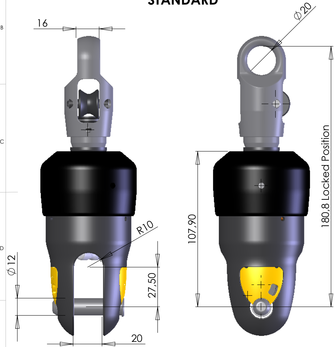
PF320600 Lashing 90° from halyard
